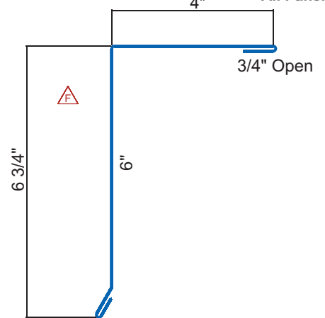
Box Gable Trim, 6-3/4" Face
