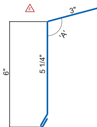
Eave Drip Edge, 6" Face For all slopes
