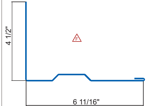
ML200 Sub-Flashing Angle For use with "stand-off" clip types
