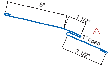
Transition Flashing For low ends of panels over membrane roofing
