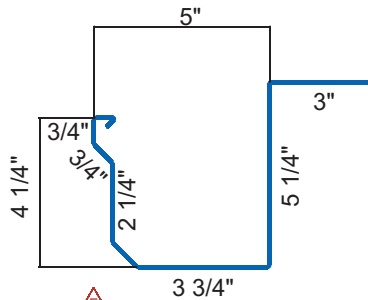
Gutter, 5" Style D Flanged Back
