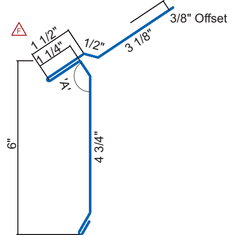
Steep Sloped Ext. Eave w/ Offset, 6" Face For slopes up to 12:12 For use with "stand-off" clip types
