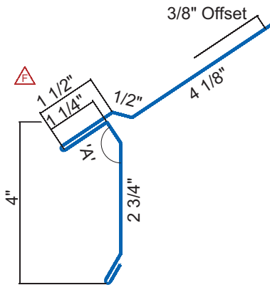
Steep Sloped Ext. Eave w/ Offset, 4" Face For slopes up to 12:12 For use with "stand-off" clip types
