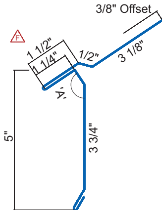
Steep Sloped Ext. Eave w/ Offset, 5" Face For slopes up to 12:12 For use with "stand-off" clip types
