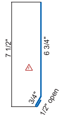
Fascia Cover, 7-1/2" w/ kickout Use with CL01 cleat
